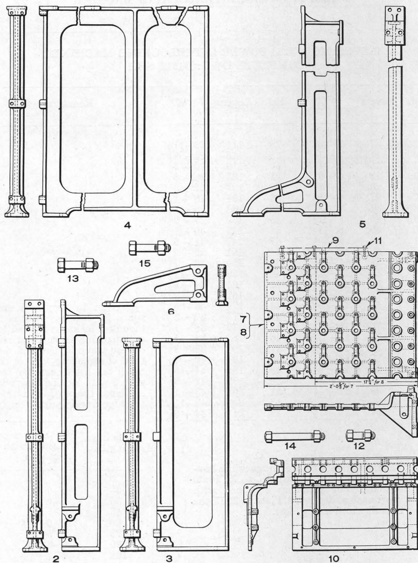
LEGS, FRONT AND BACK PLATES
